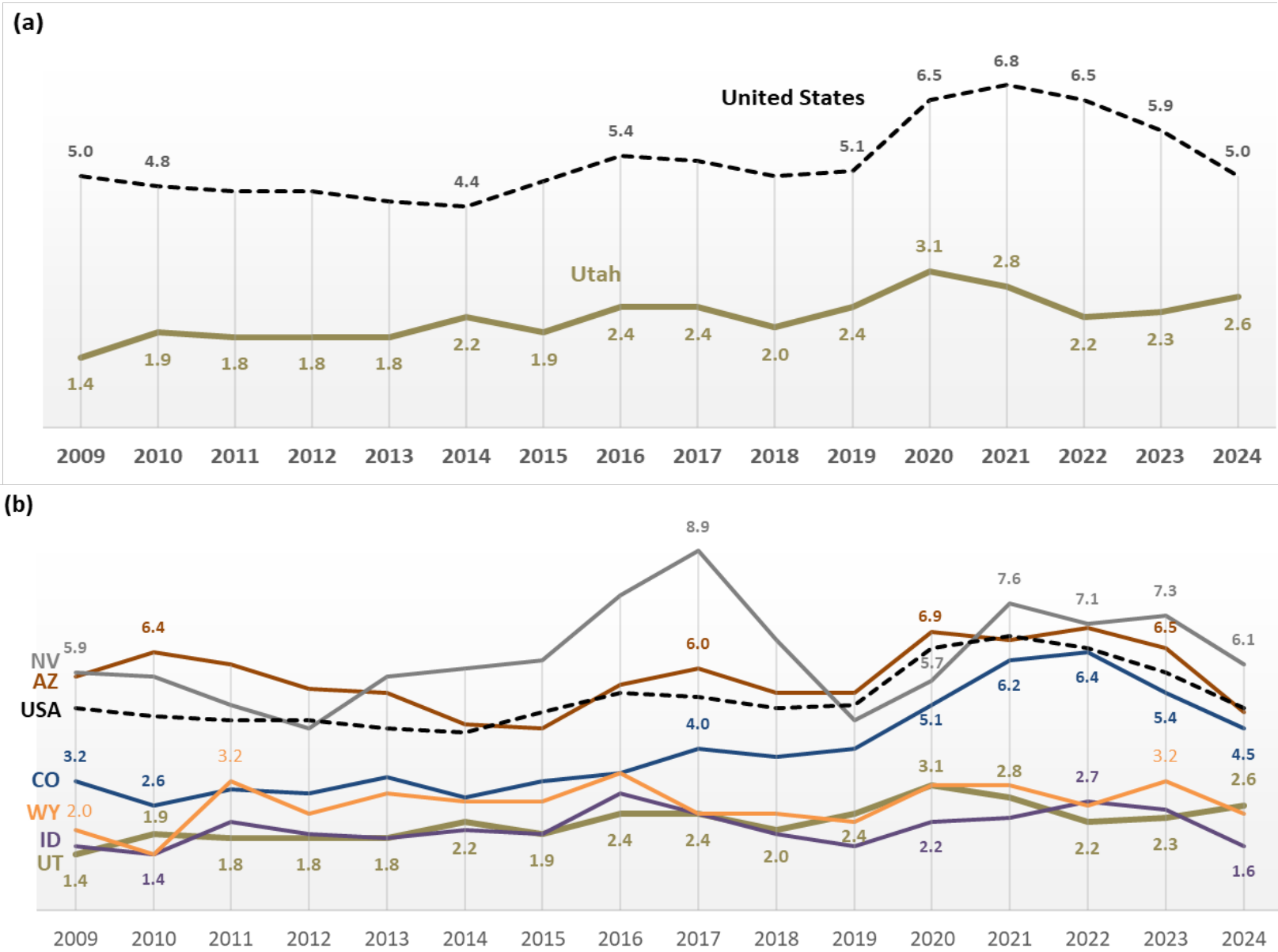
Figure O-3. FBI Uniform Crime Reporting (UCR) homicide rate (rate per 100,000 population) trends in Utah compared to national rates (a), and compared to other nearby states (b), 2009-24 ( return to p.10 ).
